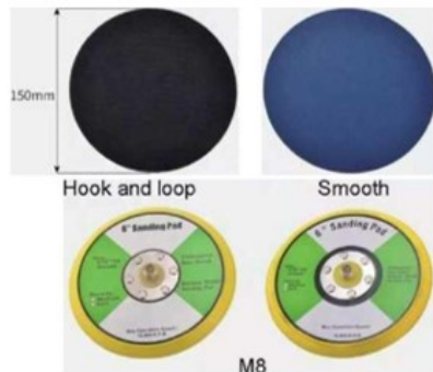
6inch 150mm M8 screw thread
